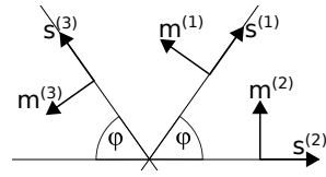
Figure 2: Scheme of slip systems
