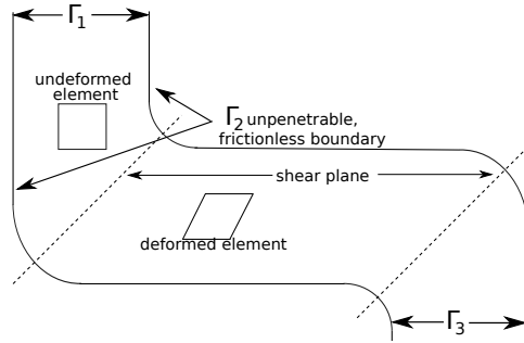
Figure 1: Scheme of 2-turn ECAE experiment
